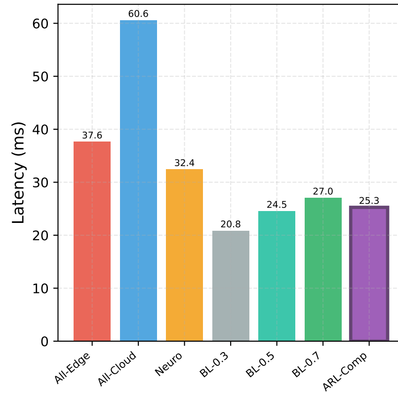
ResNet-18
