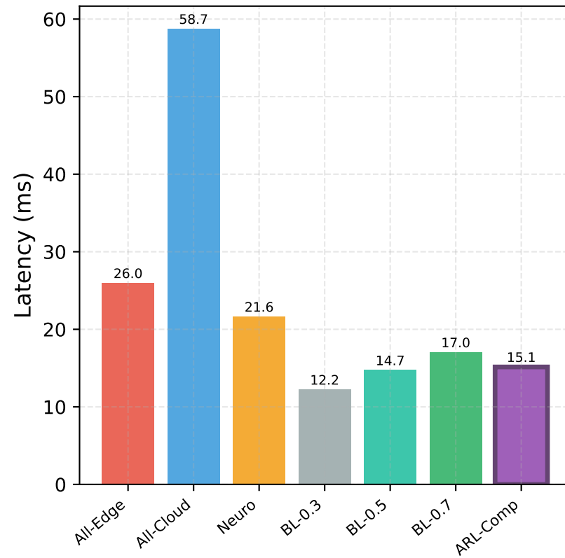
AlexNet
