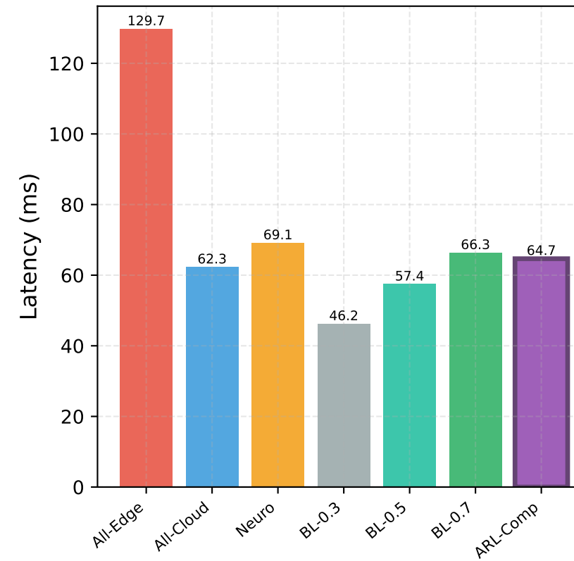
ResNet-50
