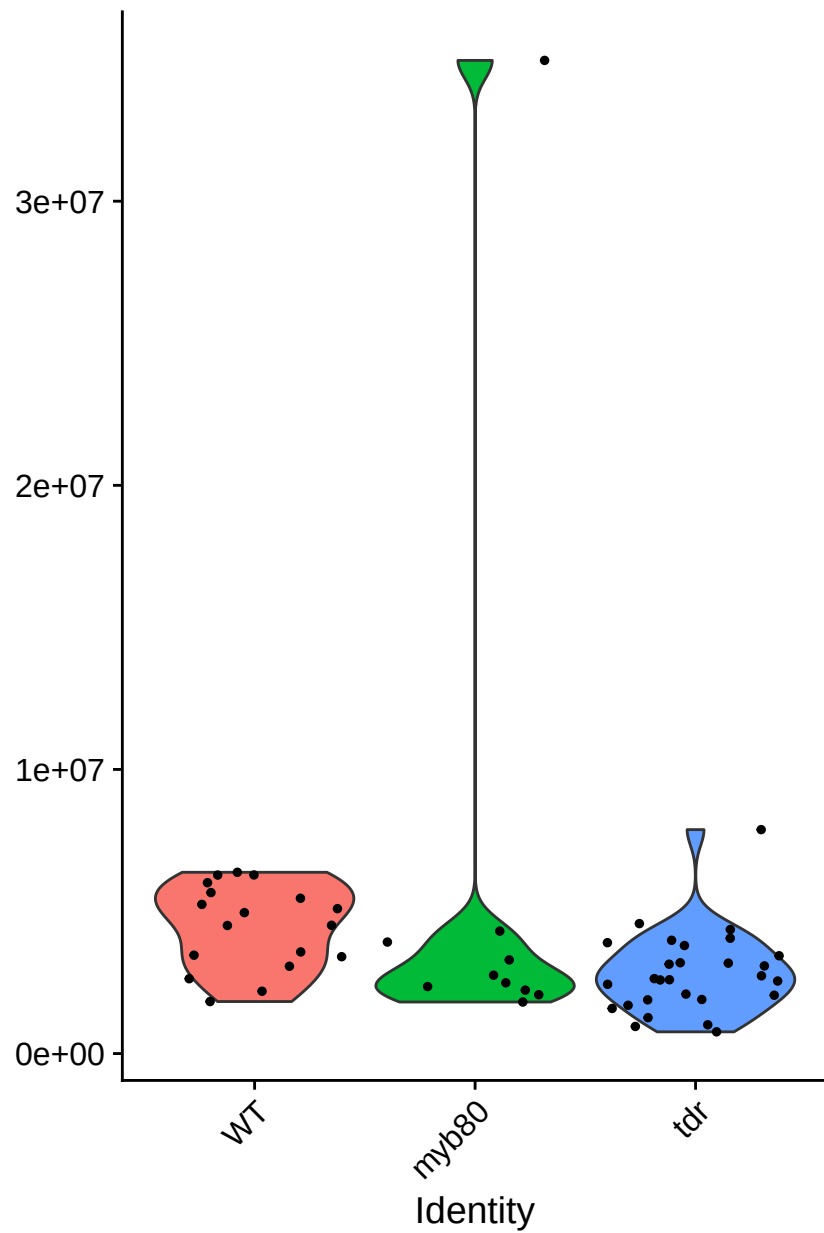
nCount_RNA
