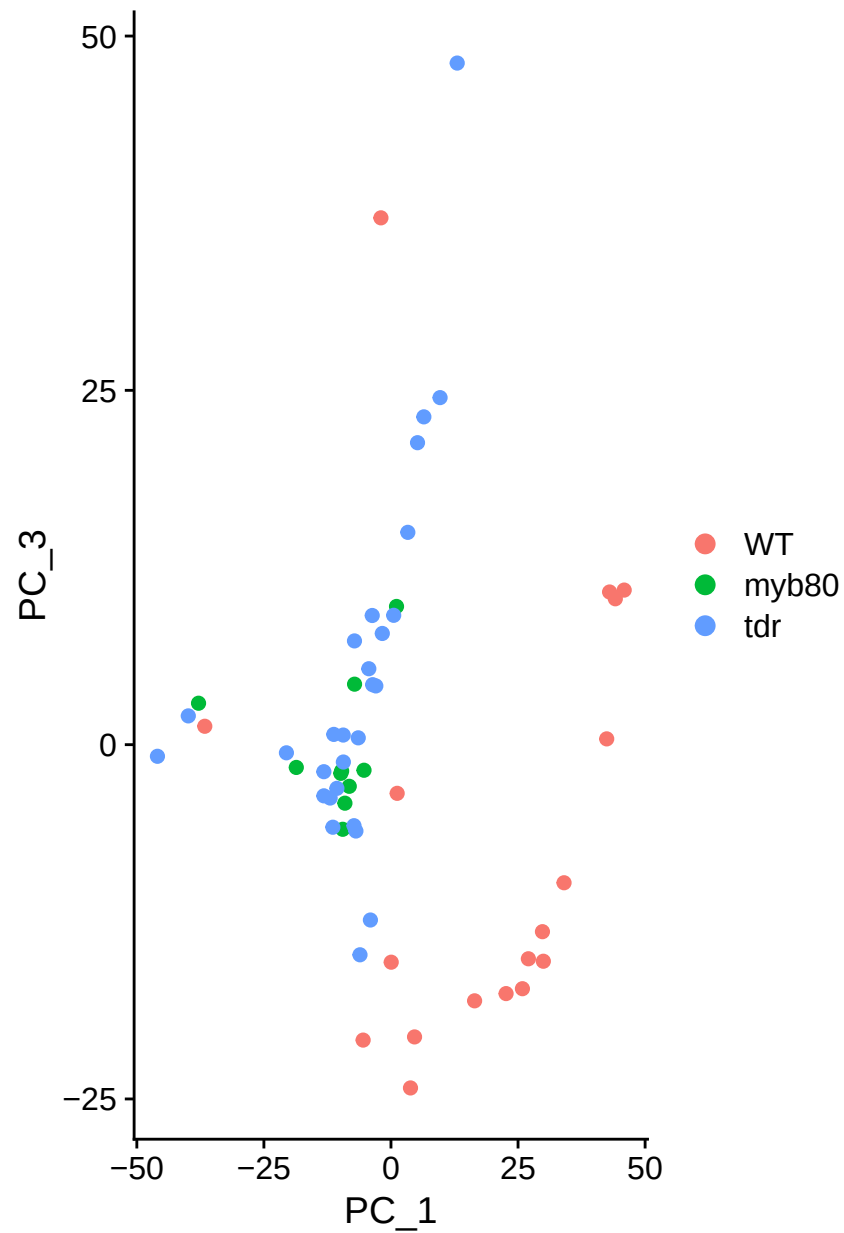
genotype
