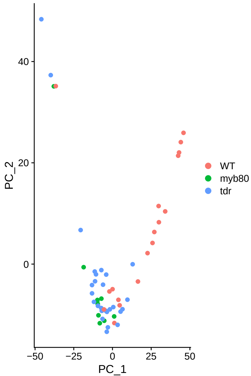
genotype
