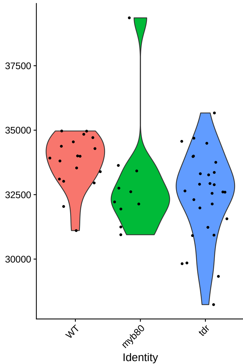
nFeature_RNA
