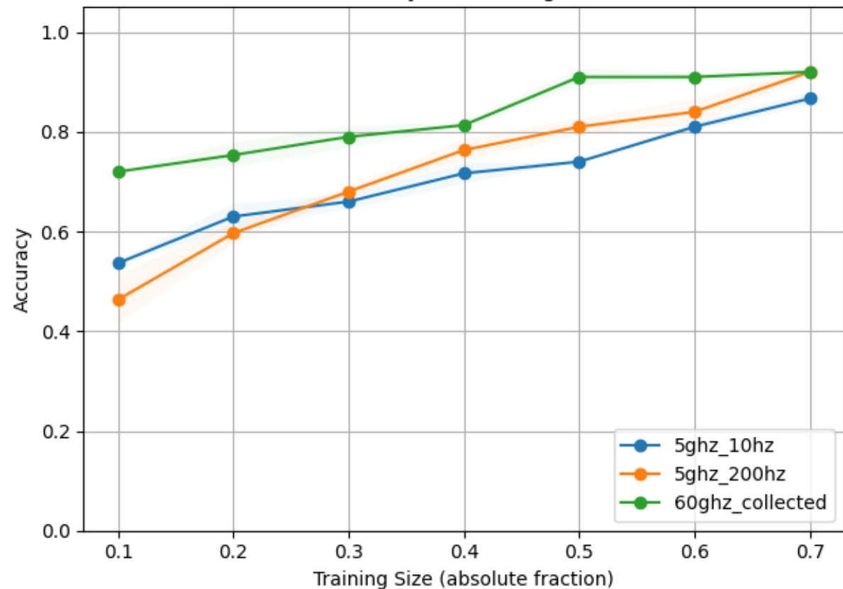
Accuracy vs. Training Size
