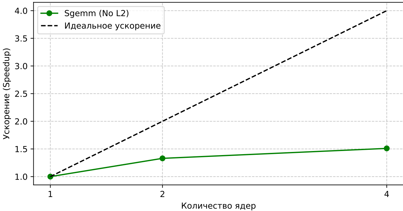
Strong Scaling: Ускорение vs Ядра (Sgemm - Compute-Bound)
