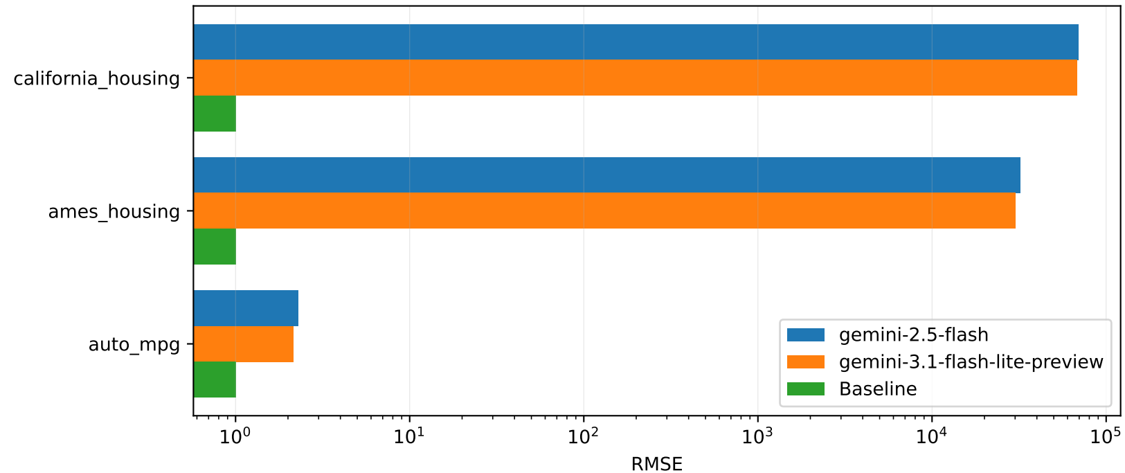
Regression performance by dataset
