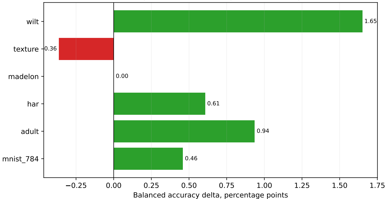
Classification delta: gemini-3.1-flash-lite-preview versus gemini-2.5-flash
