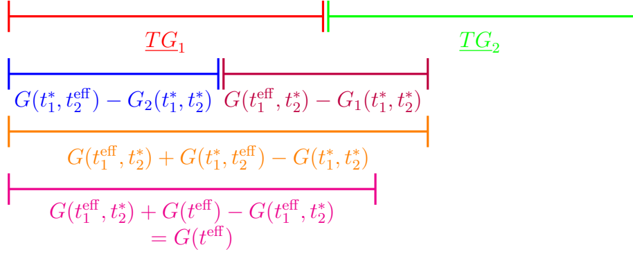
Figure 1: Impossibility under strict submodularity. Each country's pure solo claim \underline{TG}_i (top two bars) is at least what it can secure by conceding the efficient tariff to its partner while keeping its own non-cooperative tariff: the blue and purple bars are these lower bounds for countries 1 and 2. Strict submodularity makes their sum (orange) exceed the efficient surplus G(t^{\text{eff}}) (magenta), so the two claims cannot both be met and no efficient agreement is supportable.
