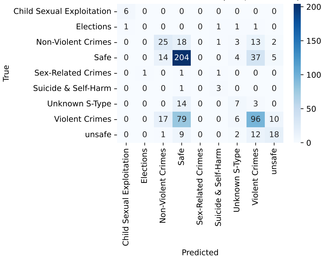
BiRNN - Confusion Matrix (Test, F1=0.435)
