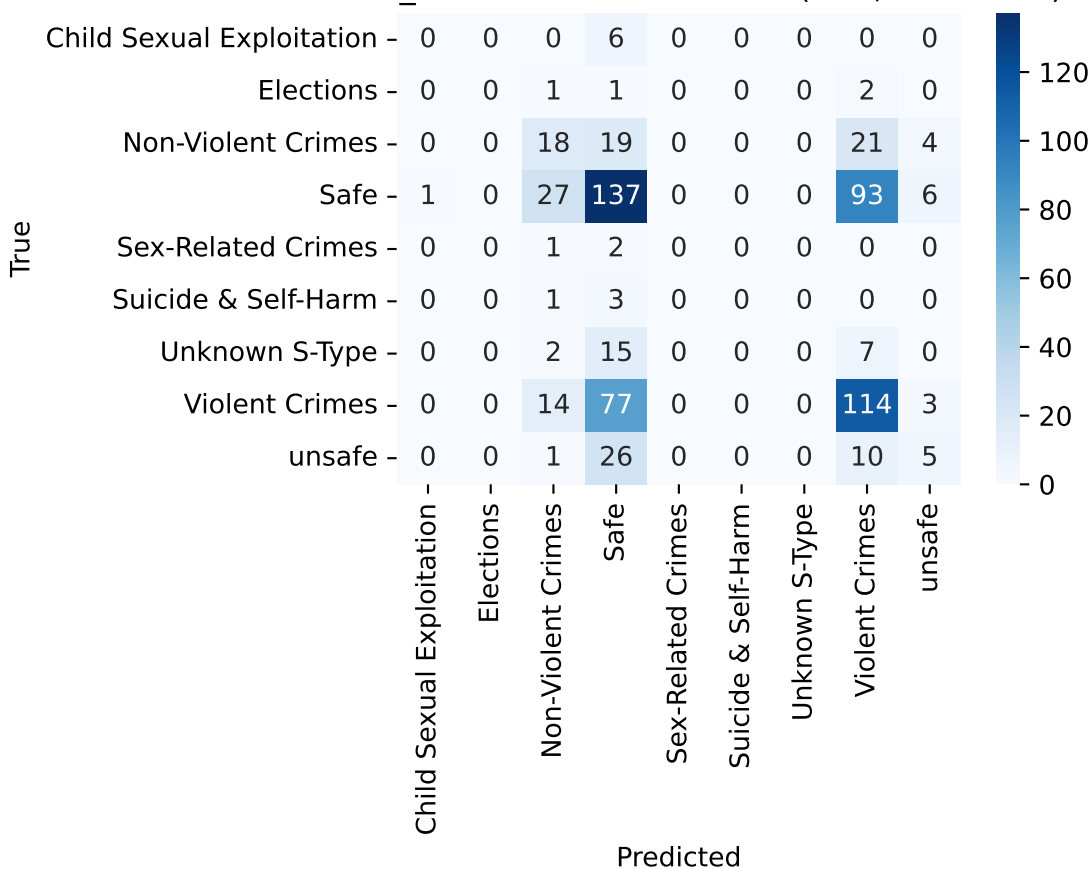
Vanilla_RNN - Confusion Matrix (Test, F1=0.161)
