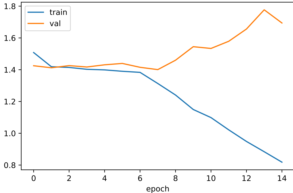
Vanilla_RNN - Loss
