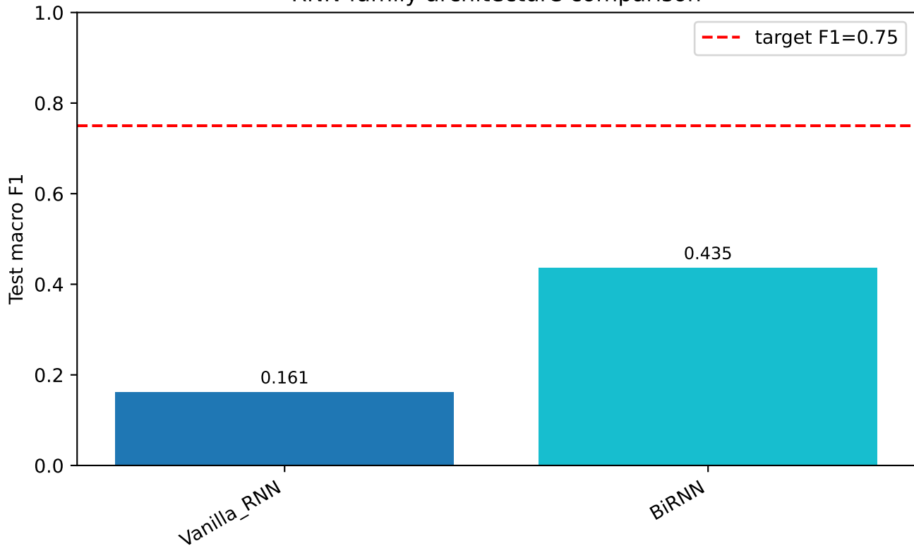
RNN-family architecture comparison
