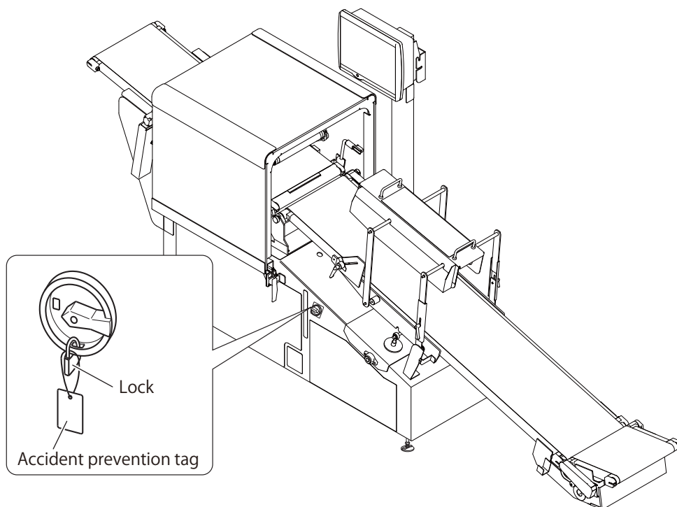
Fig.1-2 Main Power Switch
