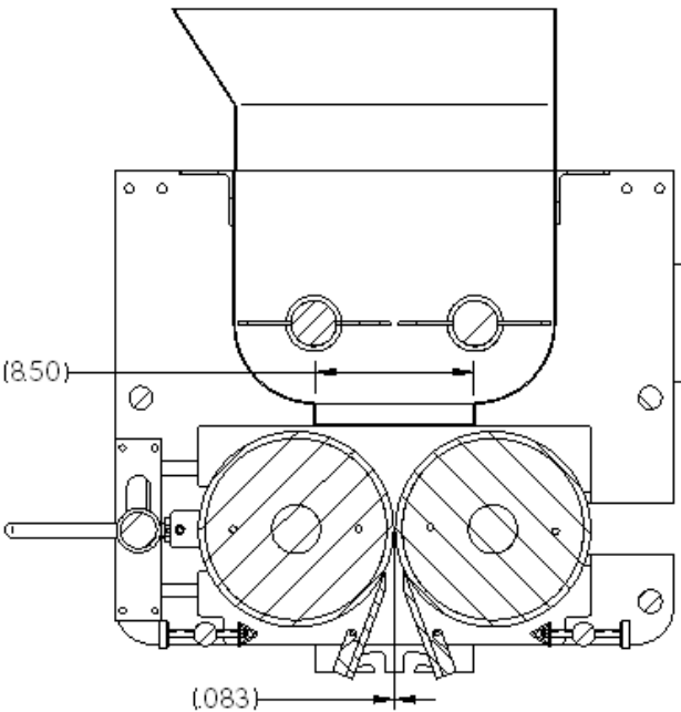
SECTION C-C
