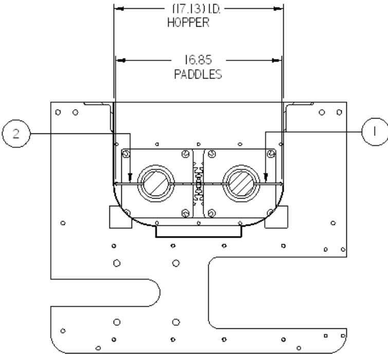
SECTION B-B
