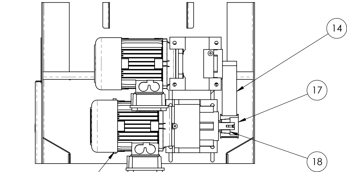
EXIT CONV MOTOR (REF) SECTION H-H
