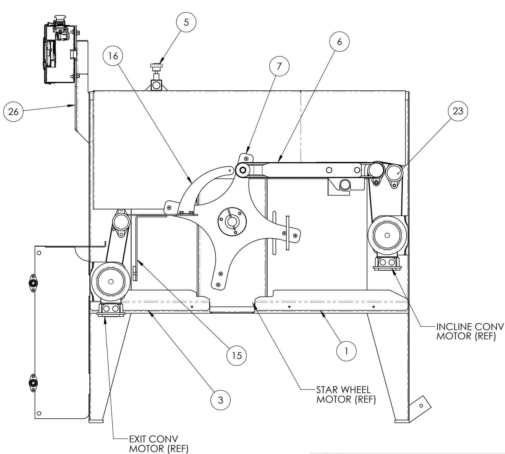
SECTION F-F
