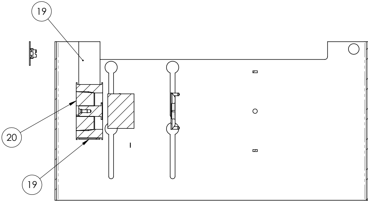
EXIT CONV MOTOR (REF) SECTION H-H
