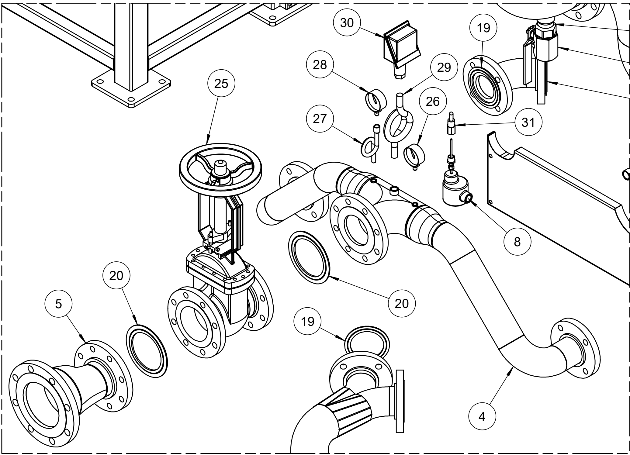
DETAIL A
