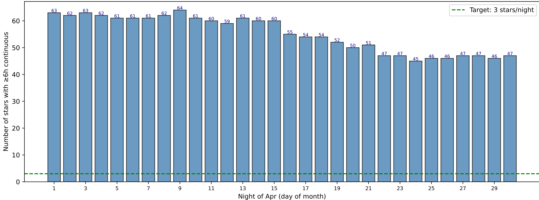
Apr 2027: OBA stars available per night (airmass \leq 2 , \geq 6.0 h continuous)
