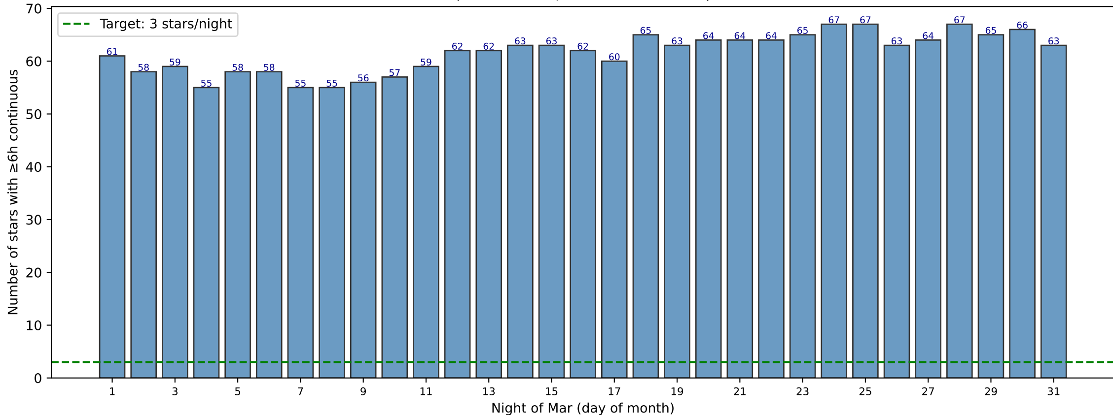
Mar 2027: OBA stars available per night (airmass \leq 2 , \geq 6.0 h continuous)
