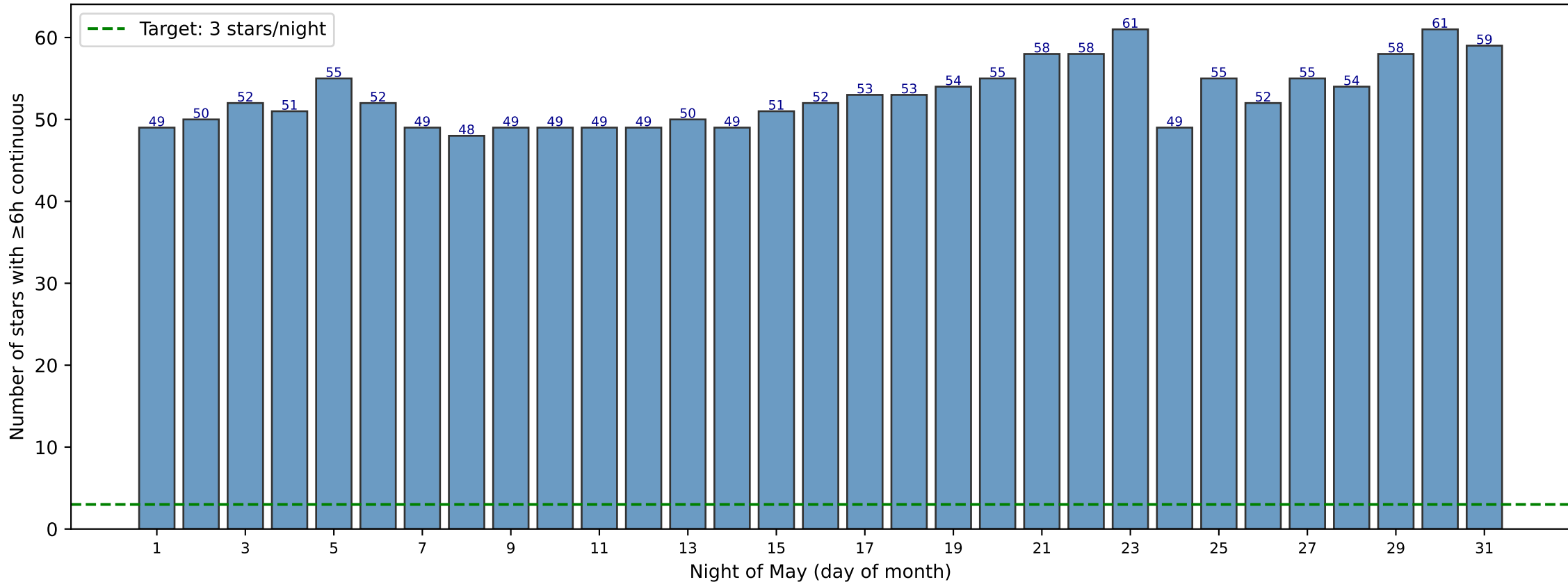
May 2027: OBA stars available per night (airmass \leq 2 , \geq 6.0 h continuous)
