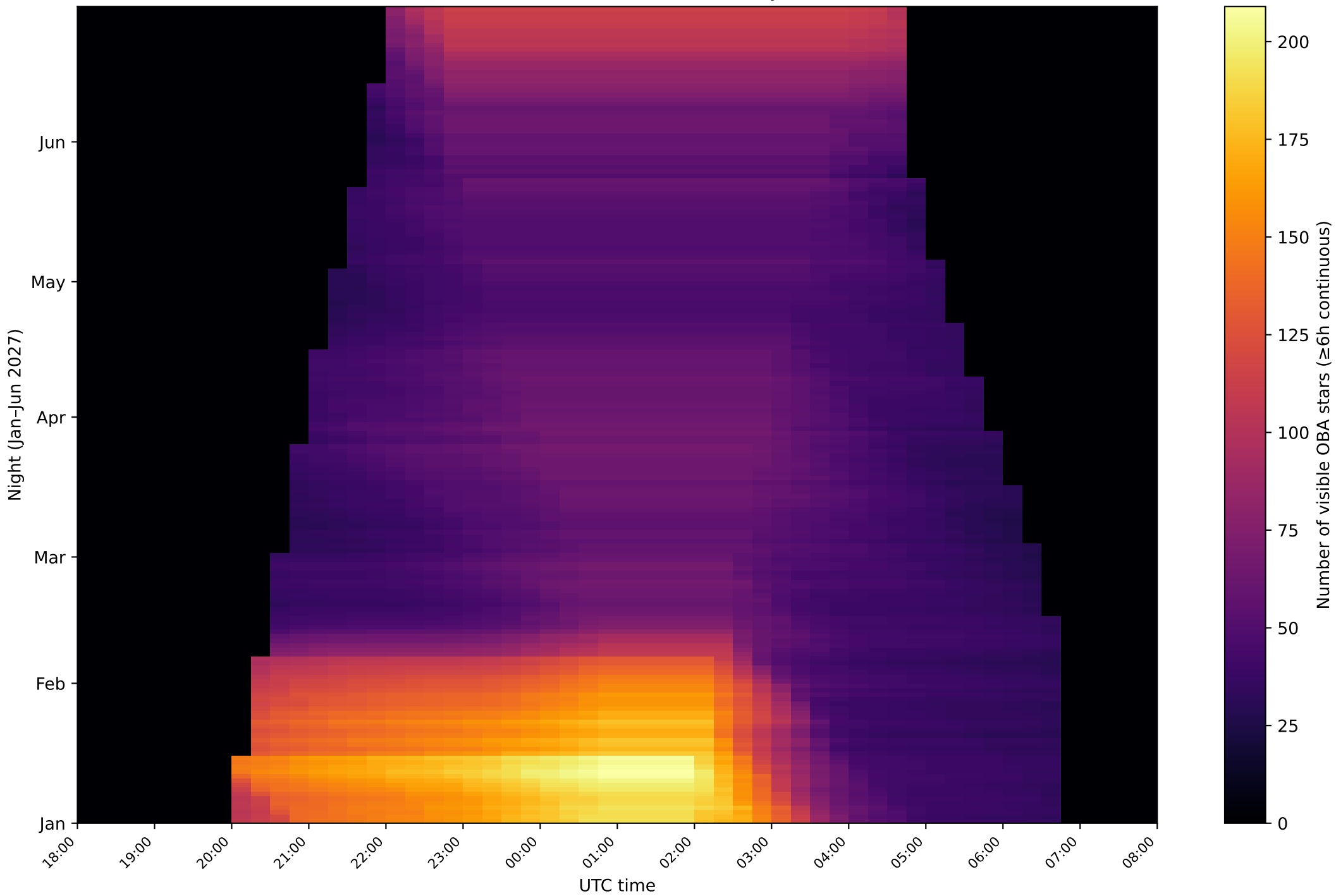
Telluric standard availability: La Palma 2027 OBA stars with \geq 6.0 h continuous observability (airmass \leq 2 )
