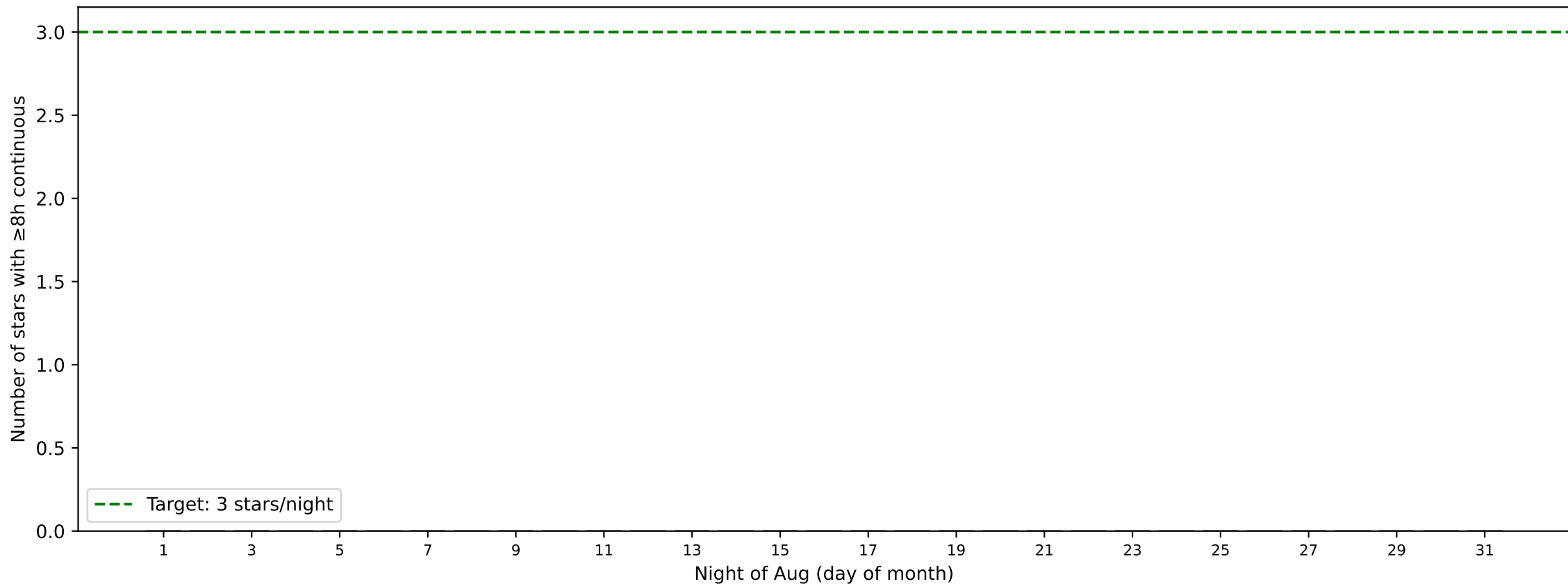
Aug 2027: OBA stars available per night (airmass \leq 1.5 , \geq 8.0 h continuous)
