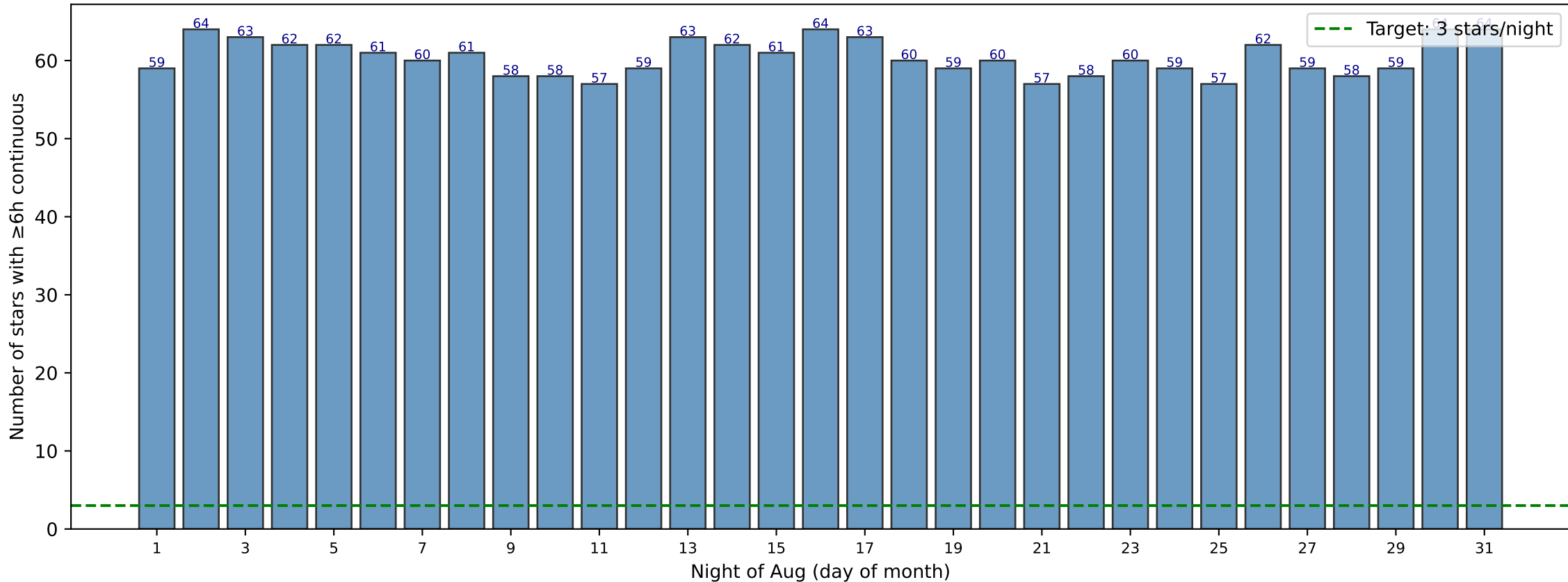
Aug 2027: OBA stars available per night (airmass \leq 1.5 , \geq 6 h continuous)
