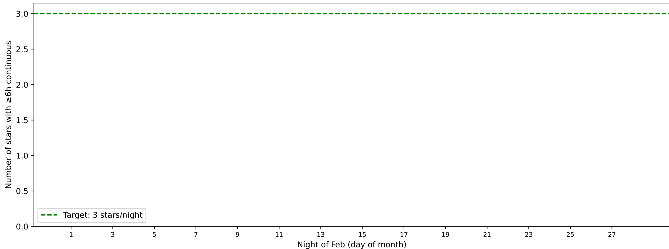
Feb 2027: OBA stars available per night (airmass \leq 1.5 , \geq 6 h continuous)
