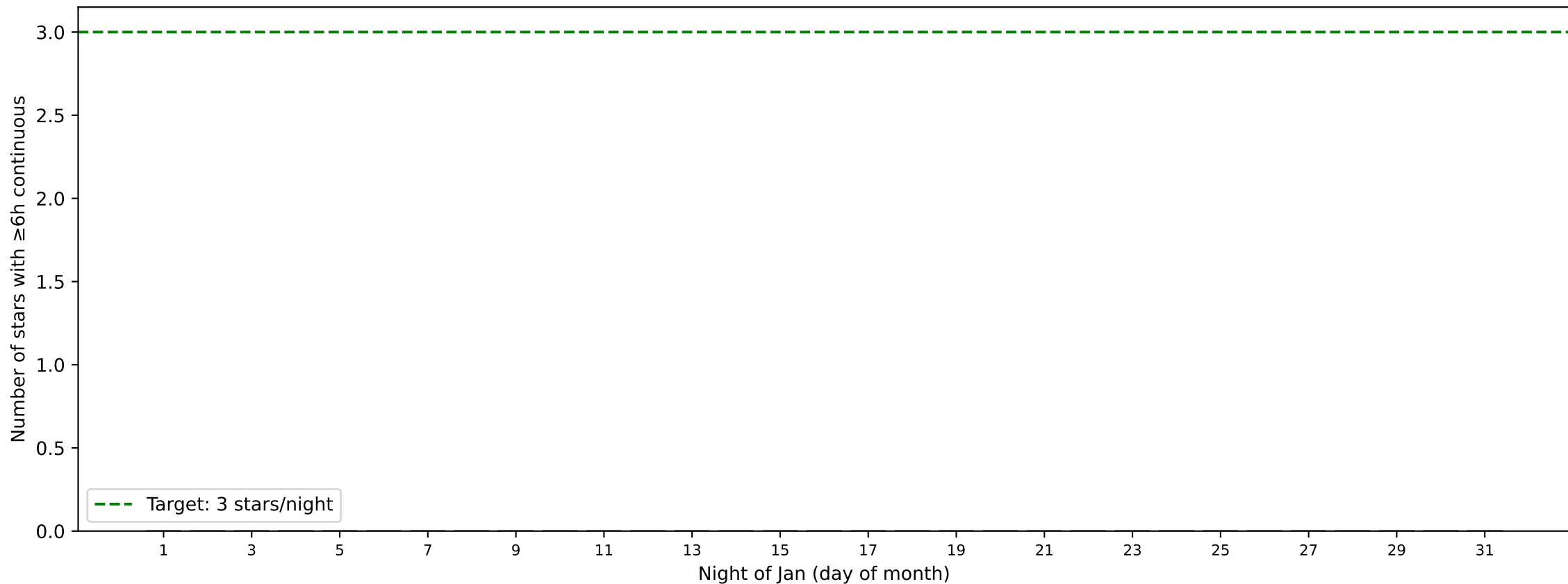
Jan 2027: OBA stars available per night (airmass \leq 1.5 , \geq 6.0 h continuous)
