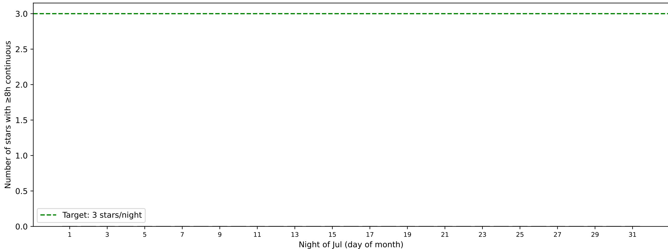
Jul 2027: OBA stars available per night (airmass \leq 1.5 , \geq 8.0 h continuous)
