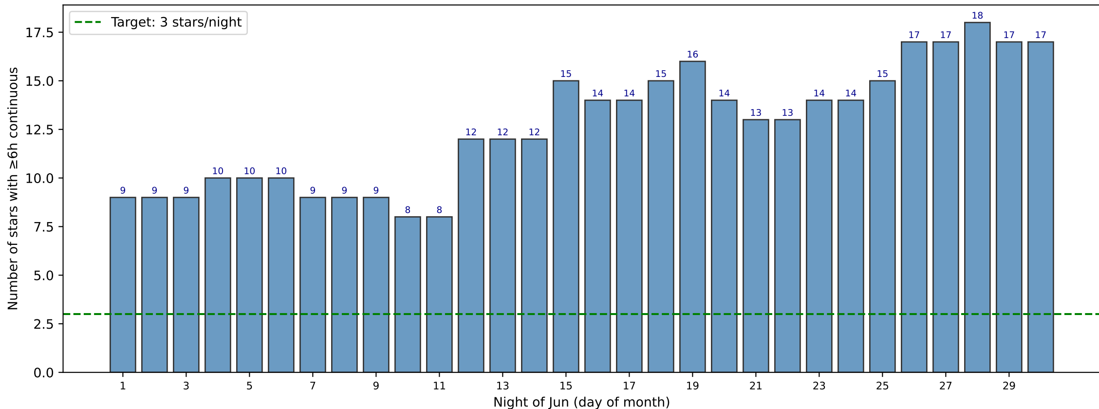
Jun 2027: OBA stars available per night (airmass \leq 1.5 , \geq 6 h continuous)
