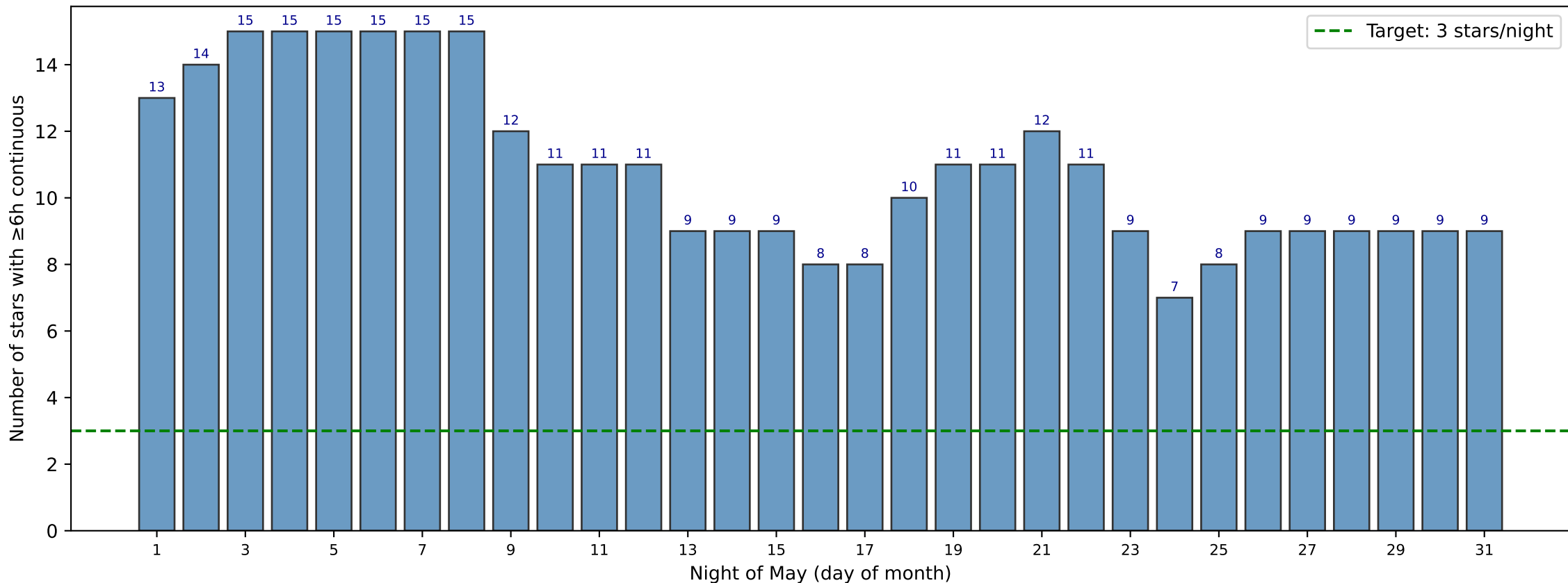
May 2027: OBA stars available per night (airmass \leq 1.5 , \geq 6 h continuous)
