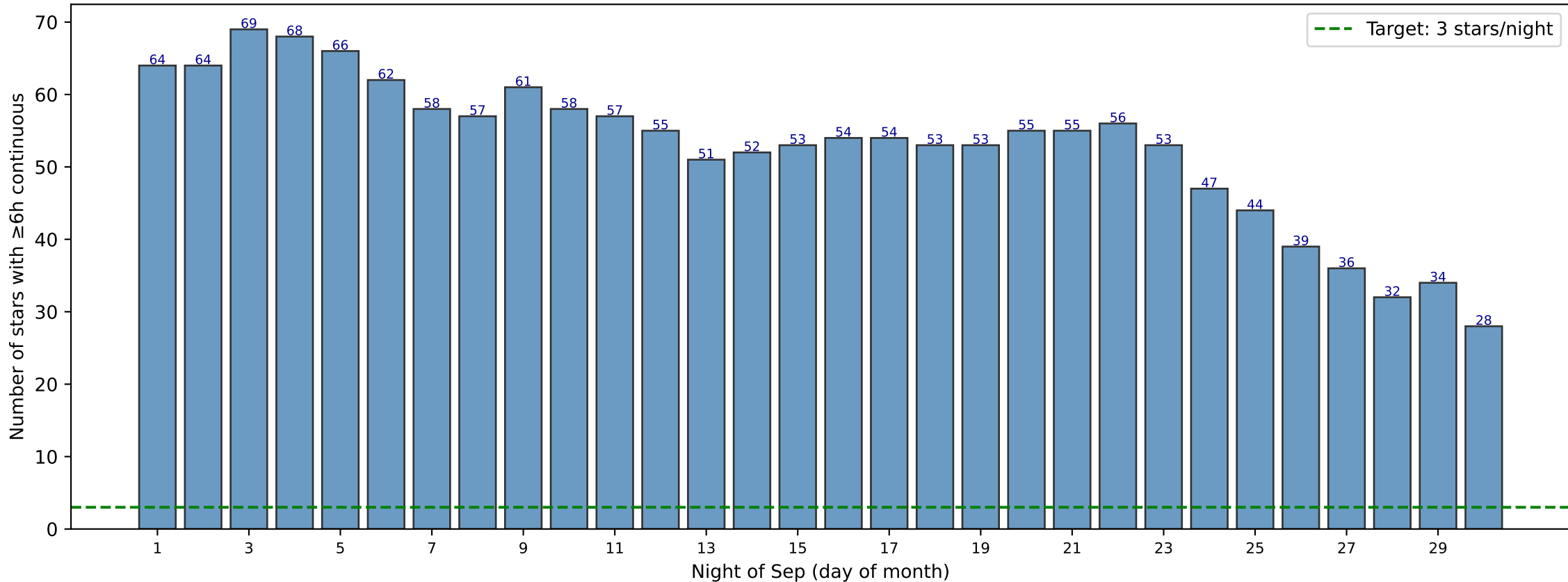
Sep 2027: OBA stars available per night (airmass \leq 1.5 , \geq 6 h continuous)
