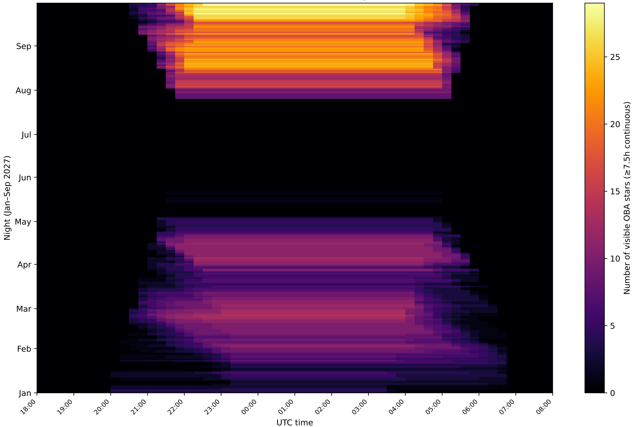
Telluric standard availability: La Palma 2027 OBA stars with \geq 7.5 h continuous observability (airmass \leq 1.5 )
