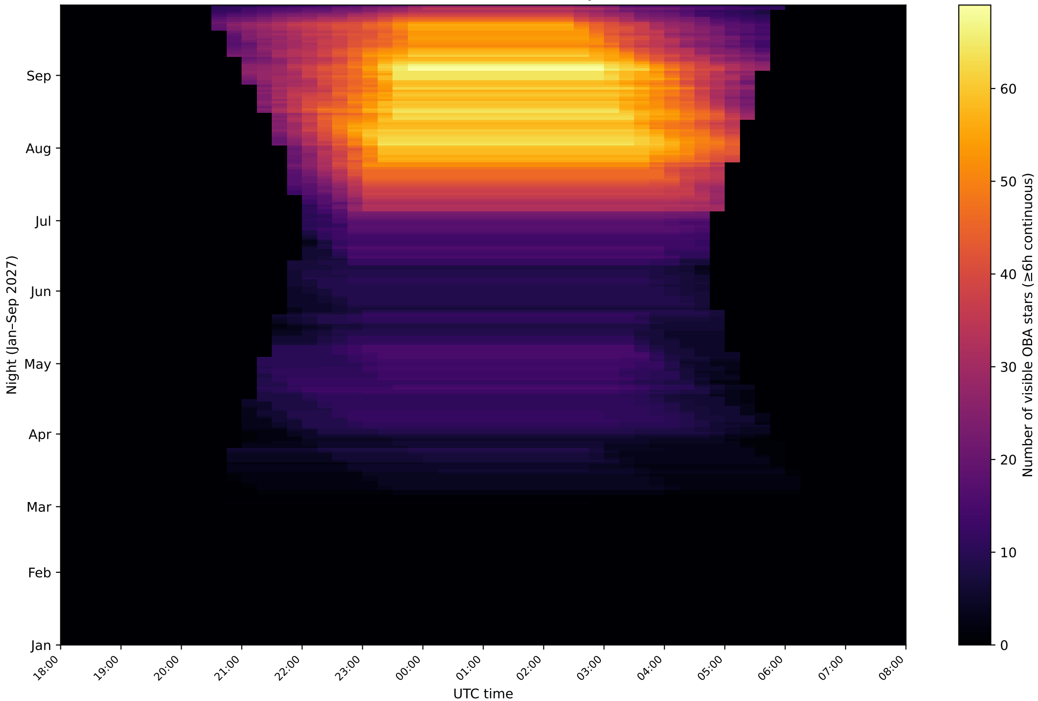
Telluric standard availability: La Palma 2027 OBA stars with \geq 6 h continuous observability (airmass \leq 1.5 )
