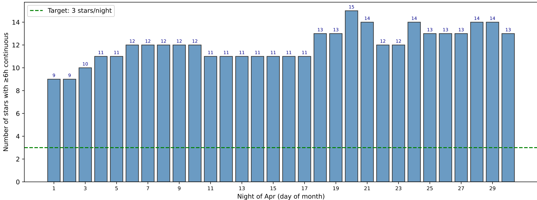
Apr 2027: OBA stars available per night (airmass \leq 1.5 , \geq 6.0 h continuous)
