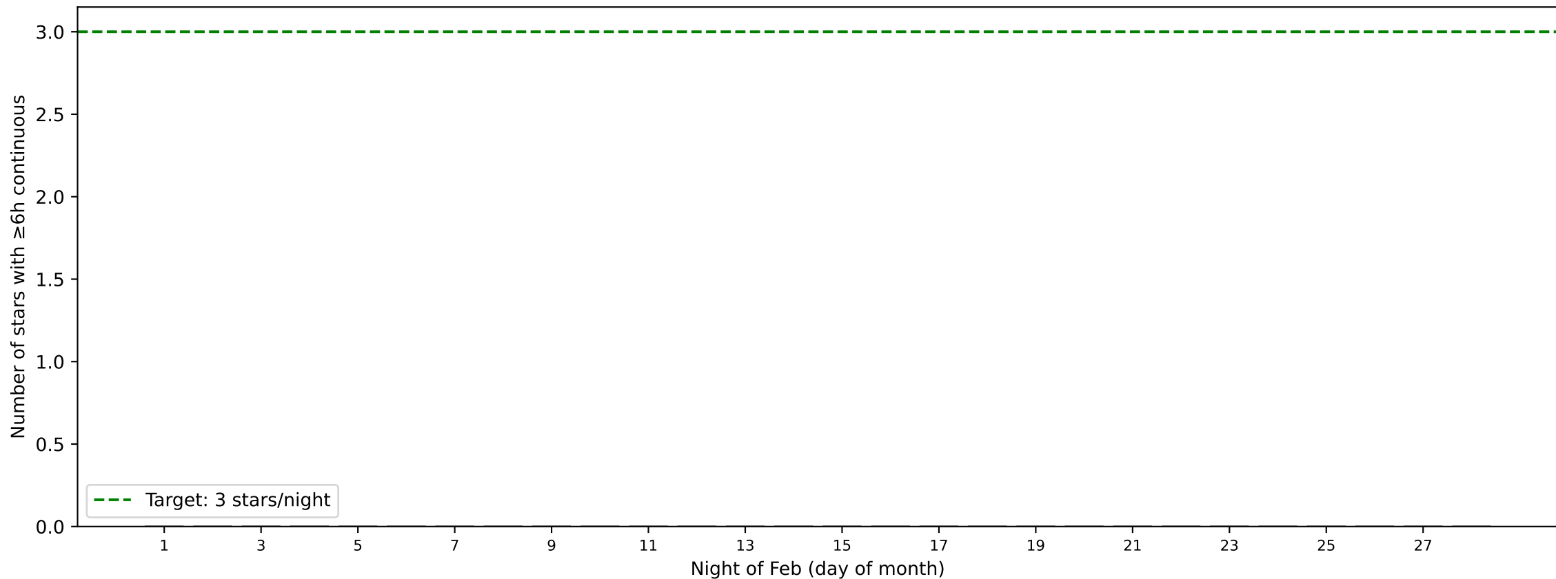
Feb 2027: OBA stars available per night (airmass \leq 1.5 , \geq 6.0 h continuous)
