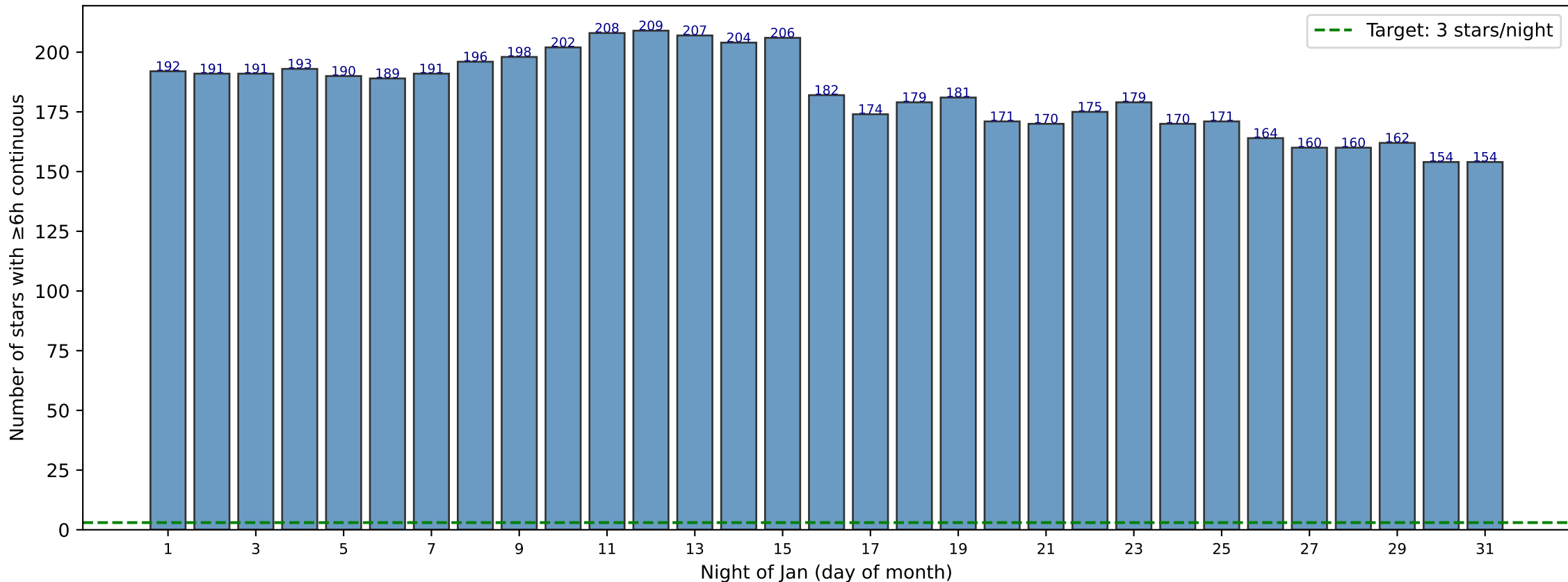
Jan 2027: OBA stars available per night (airmass \leq 2 , \geq 6.0 h continuous)
