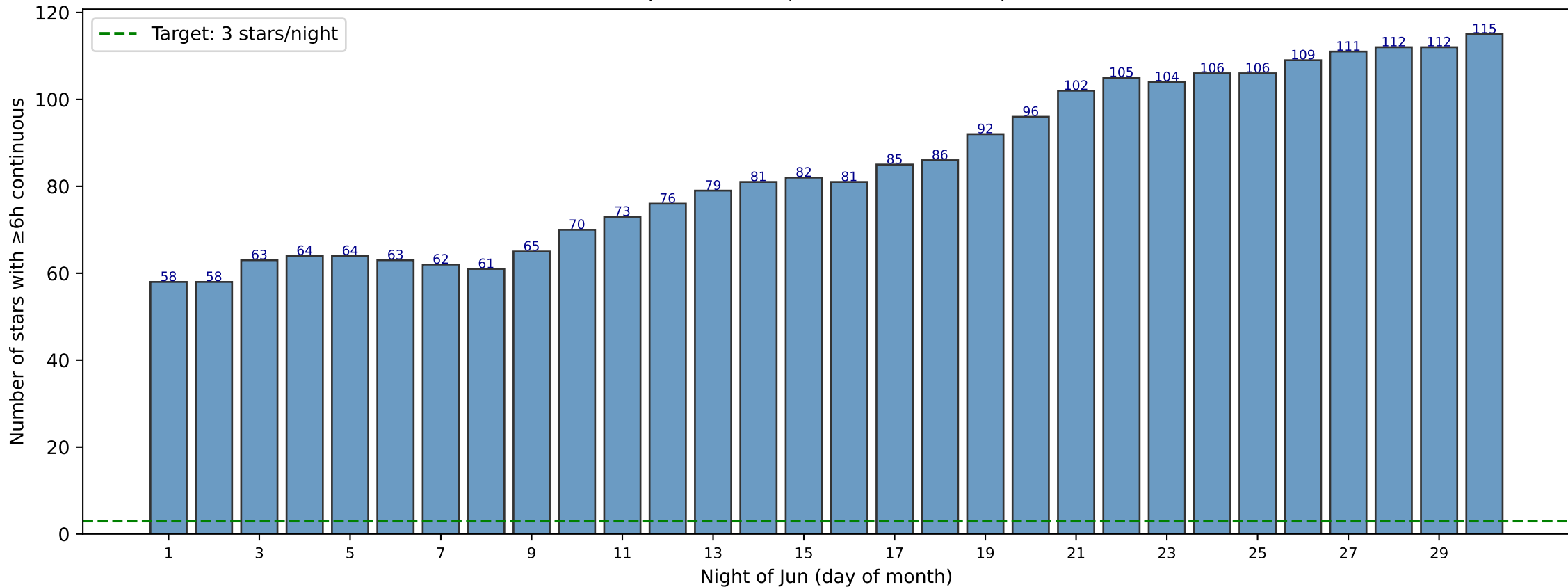
Jun 2027: OBA stars available per night (airmass \leq 2 , \geq 6.0 h continuous)
