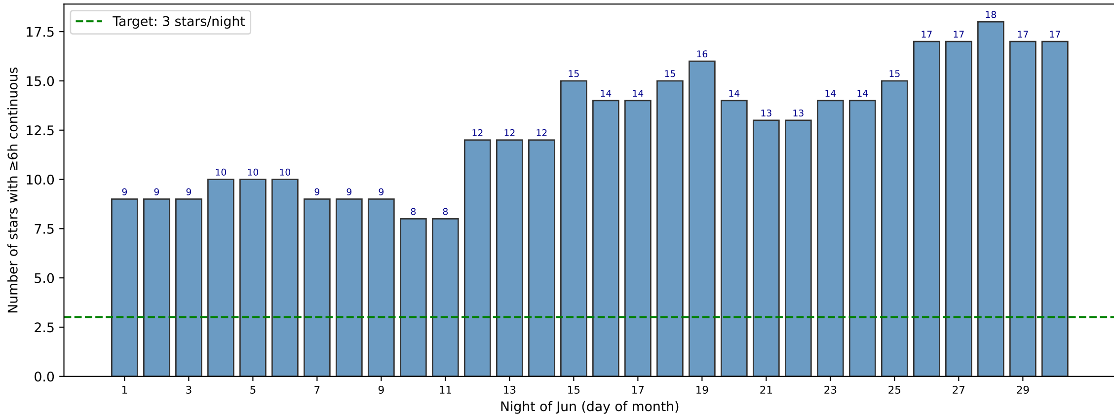
Jun 2027: OBA stars available per night (airmass \leq 1.5 , \geq 6.0 h continuous)
