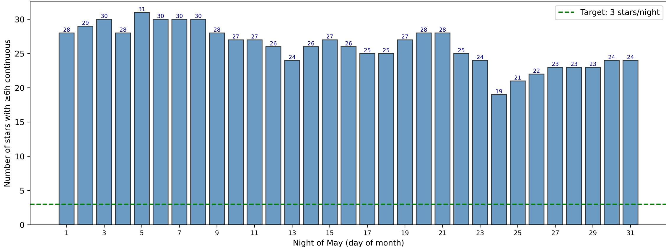
May 2027: OBA stars available per night (airmass \leq 1.5 , \geq 6.0 h continuous)
