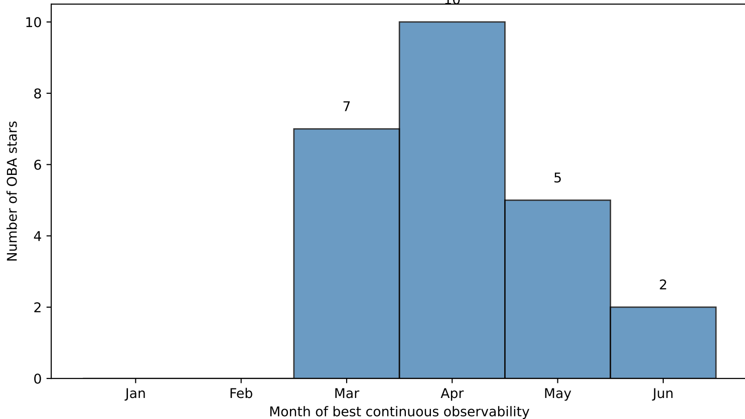
MELCHORS telluric standards: best observing month ( \geq 7.0 h continuous, airmass \leq 1.5 , La Palma 2027)
