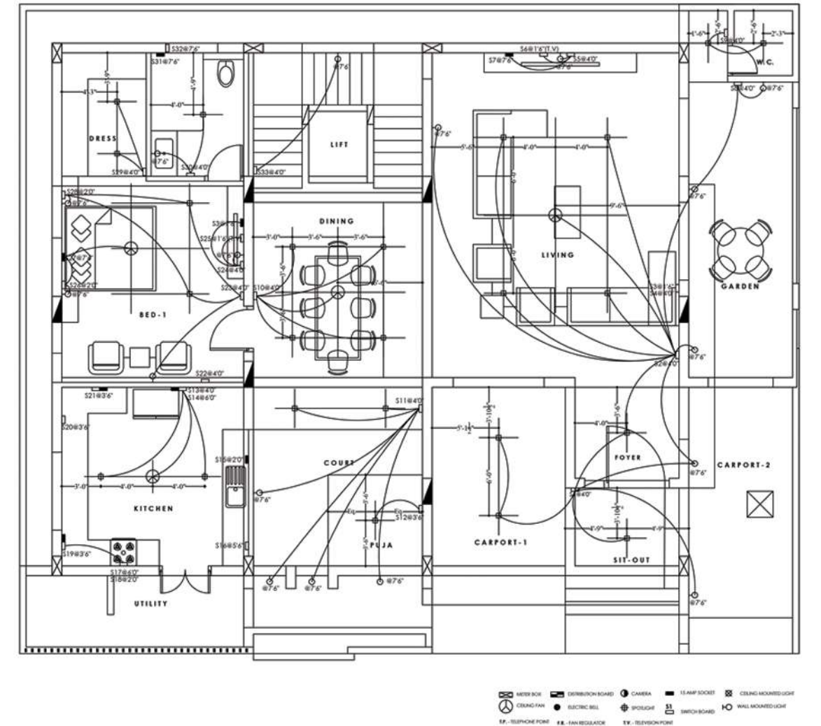
Electrical Drawing
