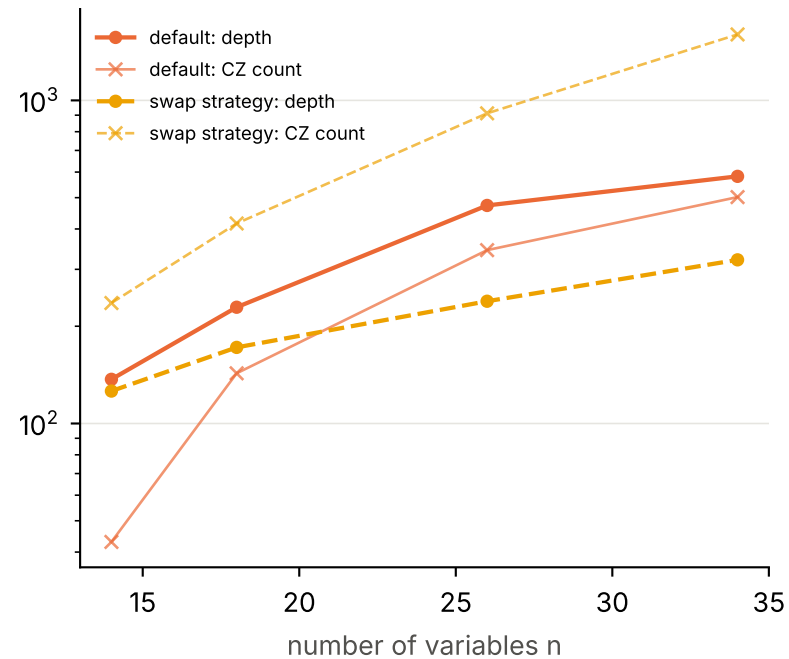
Penalty QAOA layer: SABRE vs line swap strategy
