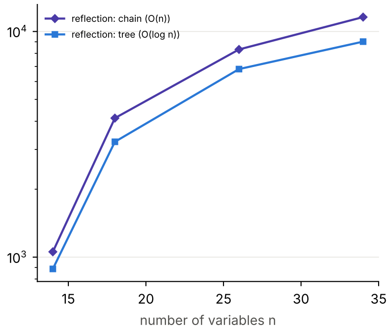
CG-QAOA layer: reflection synthesis (ibm_fez)
