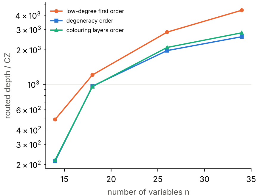
Preparation A q : vertex order (ibm_fez)
