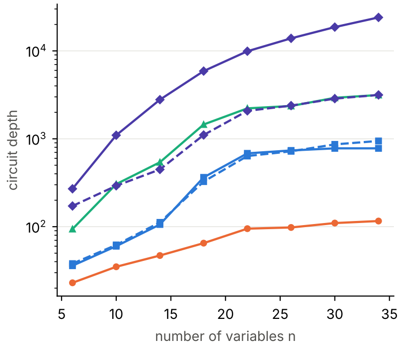
MIS (QOBLIB karate subgraphs): all-to-all
