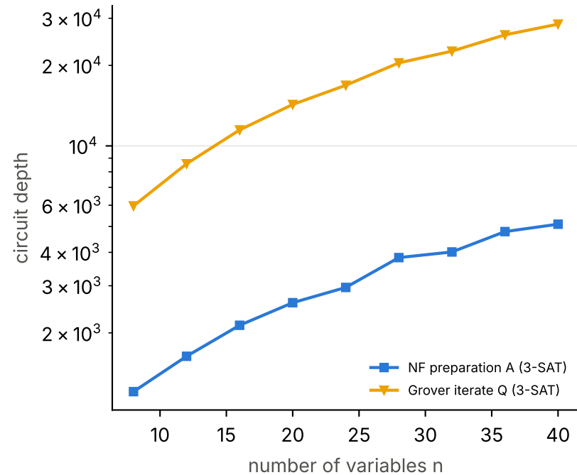
3-SAT (density 4.2): all-to-all
