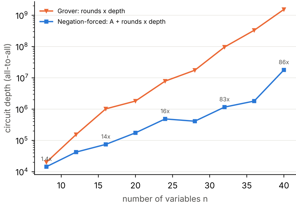
Total depth to reach a solution (median of 3 instances)
