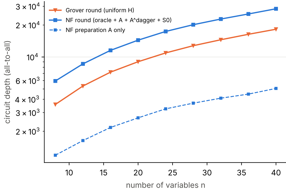
Depth of one amplification round (3-SAT)
