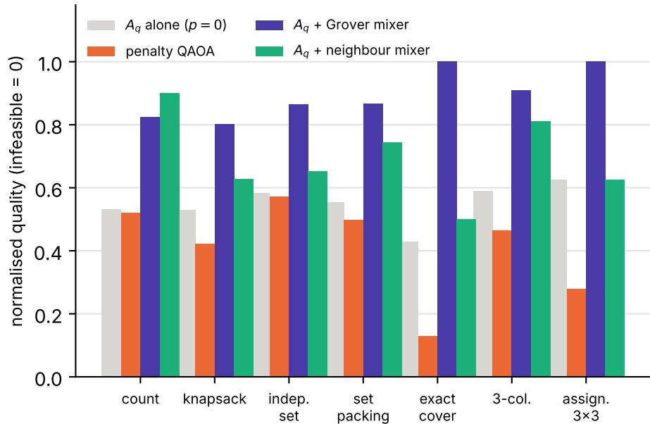
(b) QAOA, p = 3
