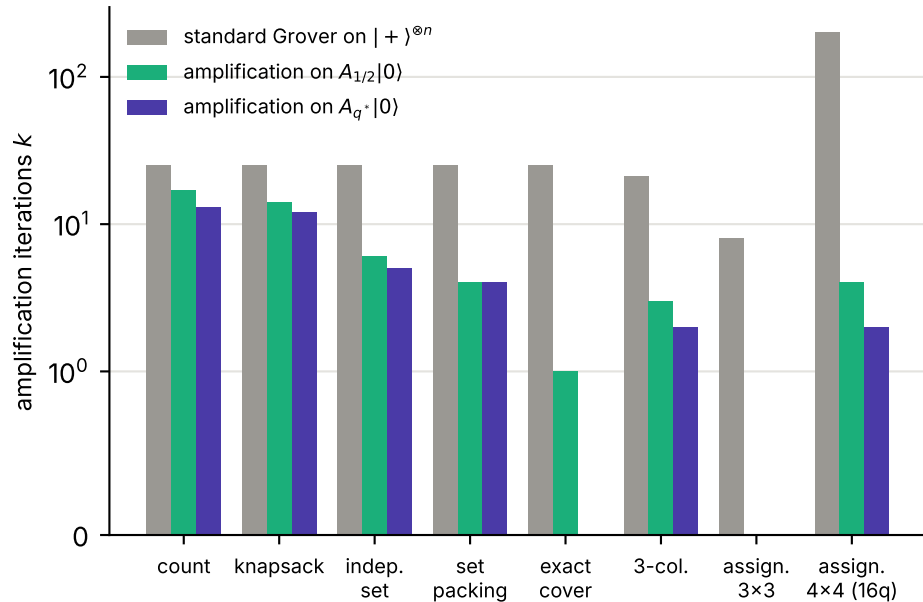
(a) Grover: iterations to find an optimum
