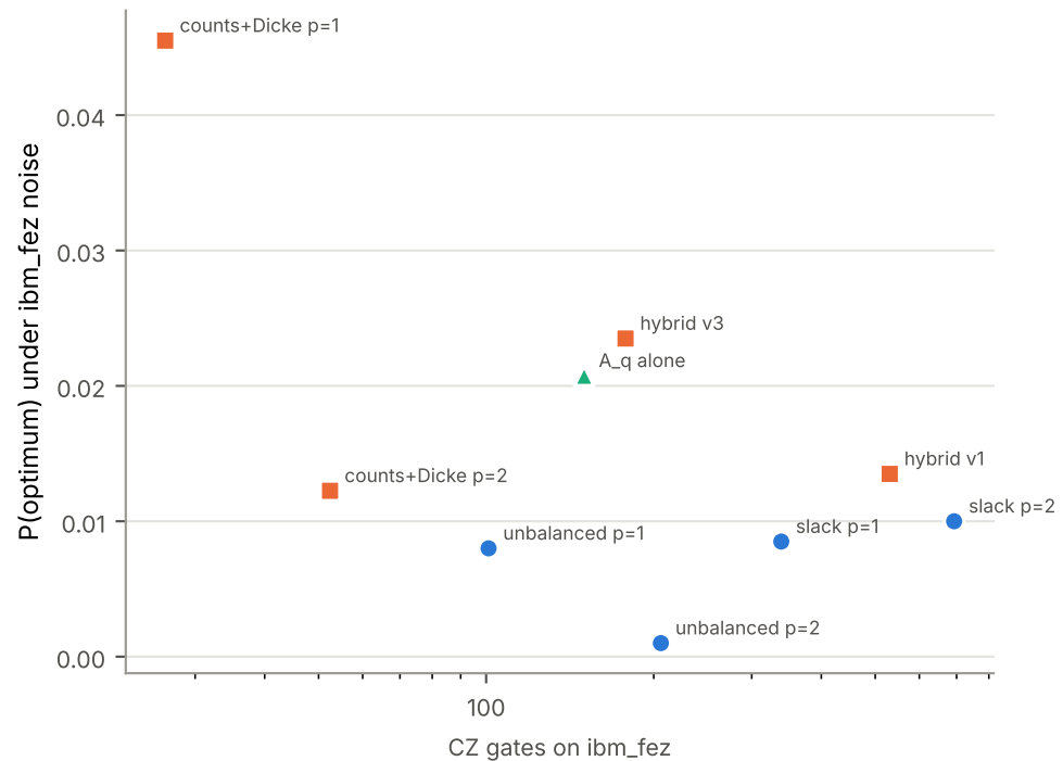
po_a003_t02_orig, ibm_fez noise model (FakeFez), 2000–4000 shots
