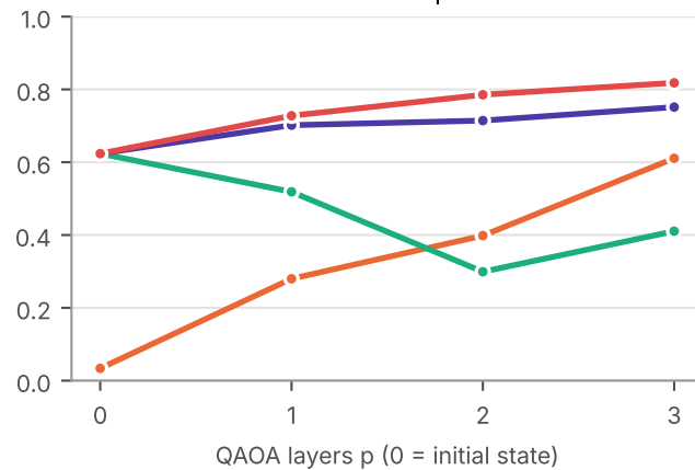
po_a005_t04_orig (2 periods) 20 decision qubits
