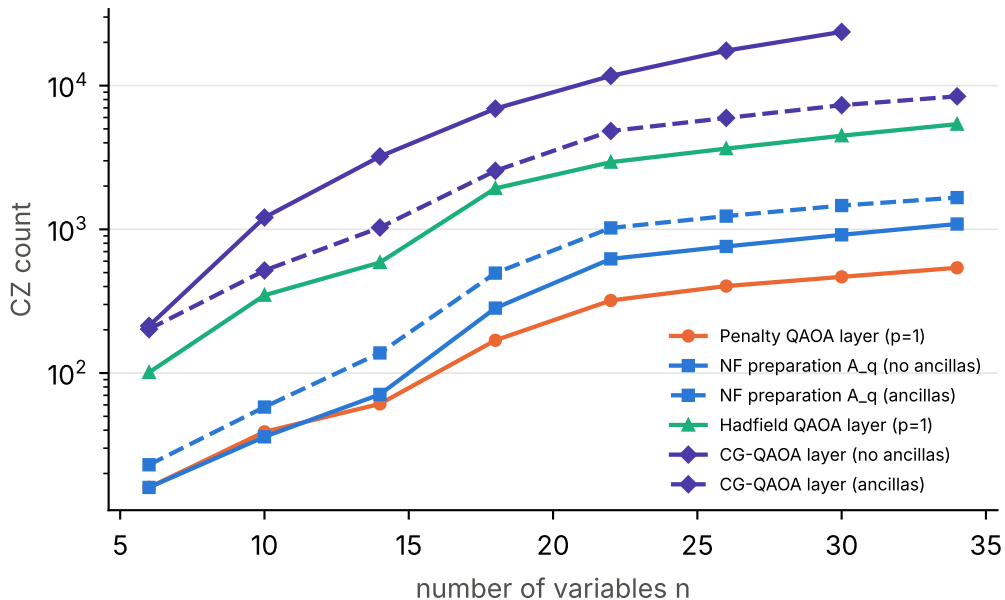
MIS: two-qubit gates on ibm_fez
