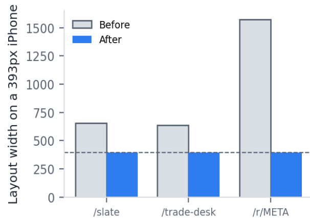
Figure 2. Before, one wide element made iOS zoom the whole page out — dock included — on Slate, Trade Desk and research. Overflow is now contained at the shell, so wide tables scroll inside their own panel.
