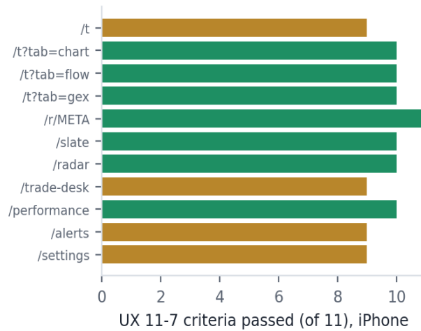
Figure 3. Final scorecard per screen on iPhone. The remaining failure on nearly every data screen is U8 (speed); fit, navigation, legibility, targets, names, honesty and titles pass.
