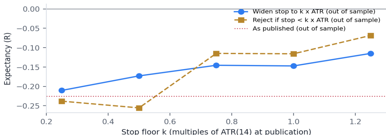
Figure 1. Out-of-sample expectancy by floor. Both interventions beat the published stops at every floor above 0.5x ATR.
