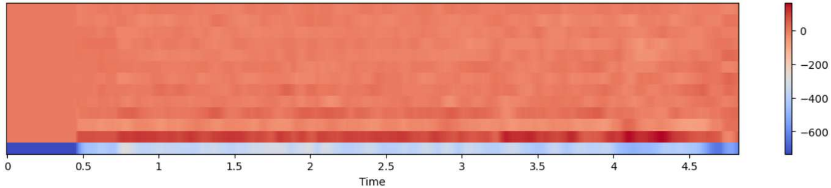
MFCC Features
