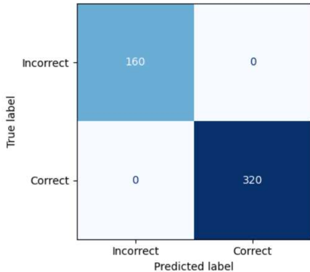
Confusion Matrix - SVM
