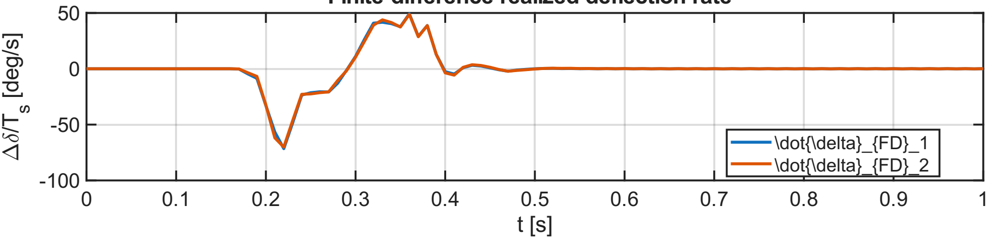
Finite-difference realized deflection rate
