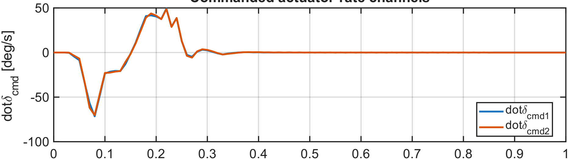
Commanded actuator-rate channels
