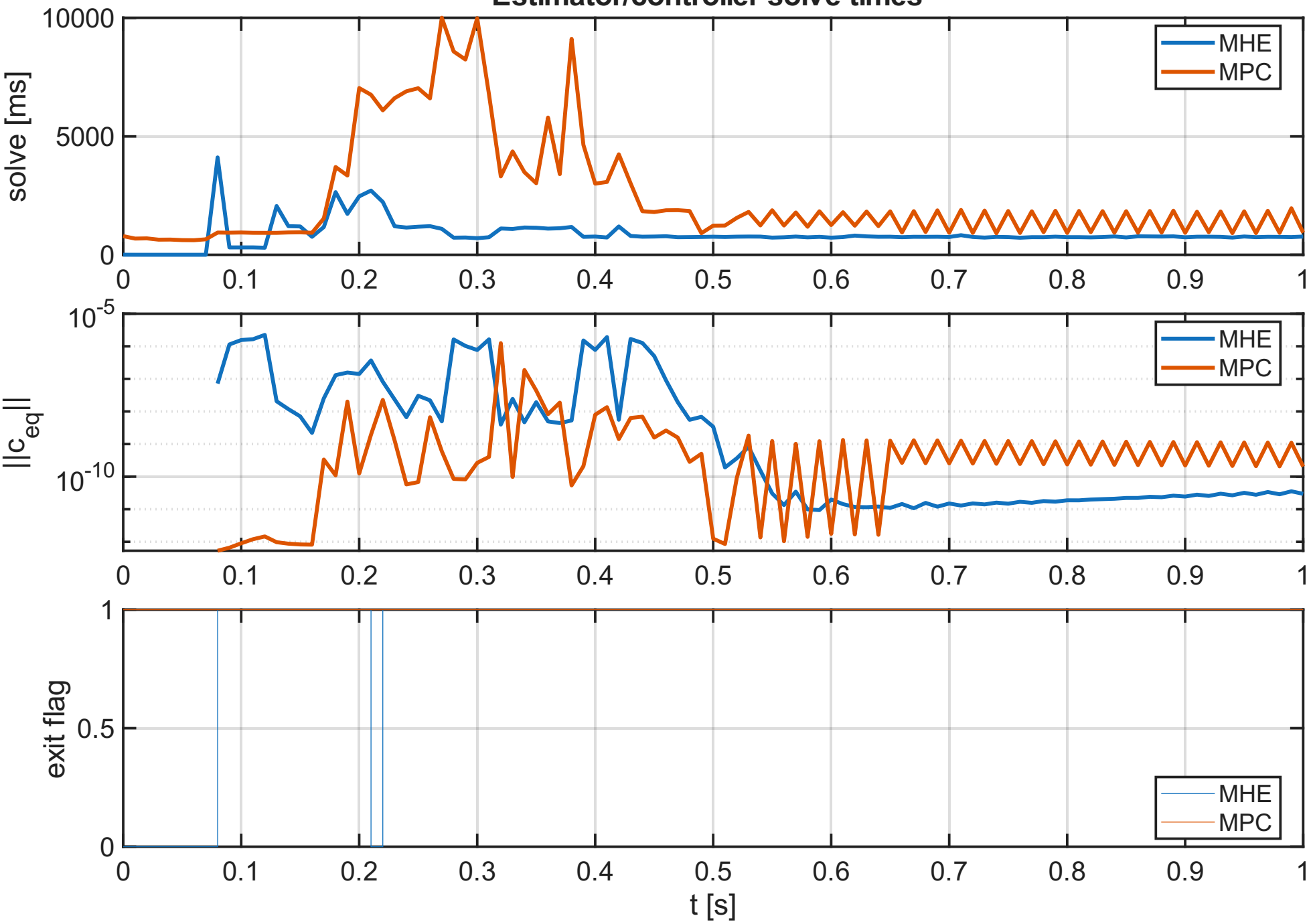
Estimator/controller solve times
