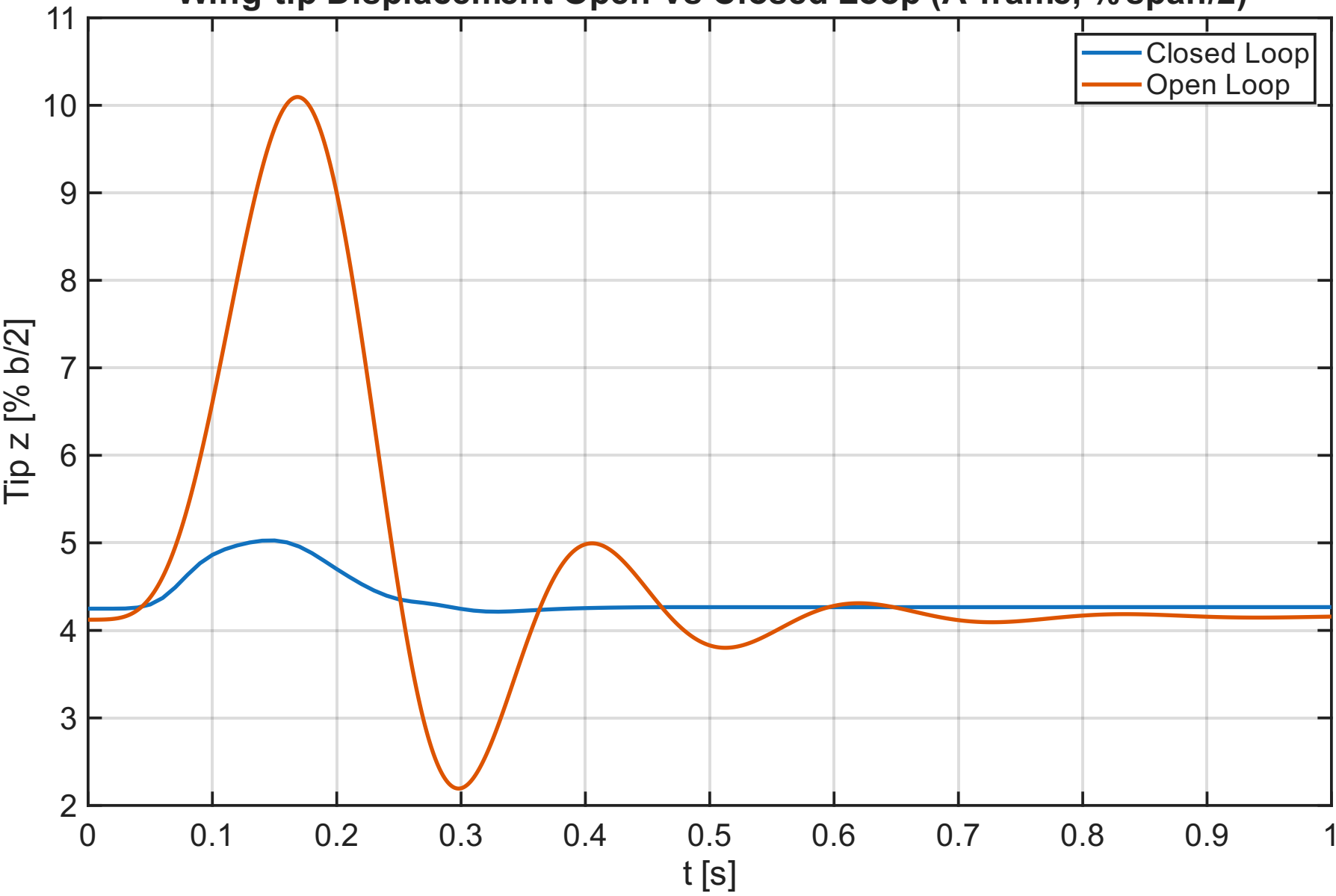
Wing-tip Displacement Open Vs Closed Loop (A-frame, % span/2)
