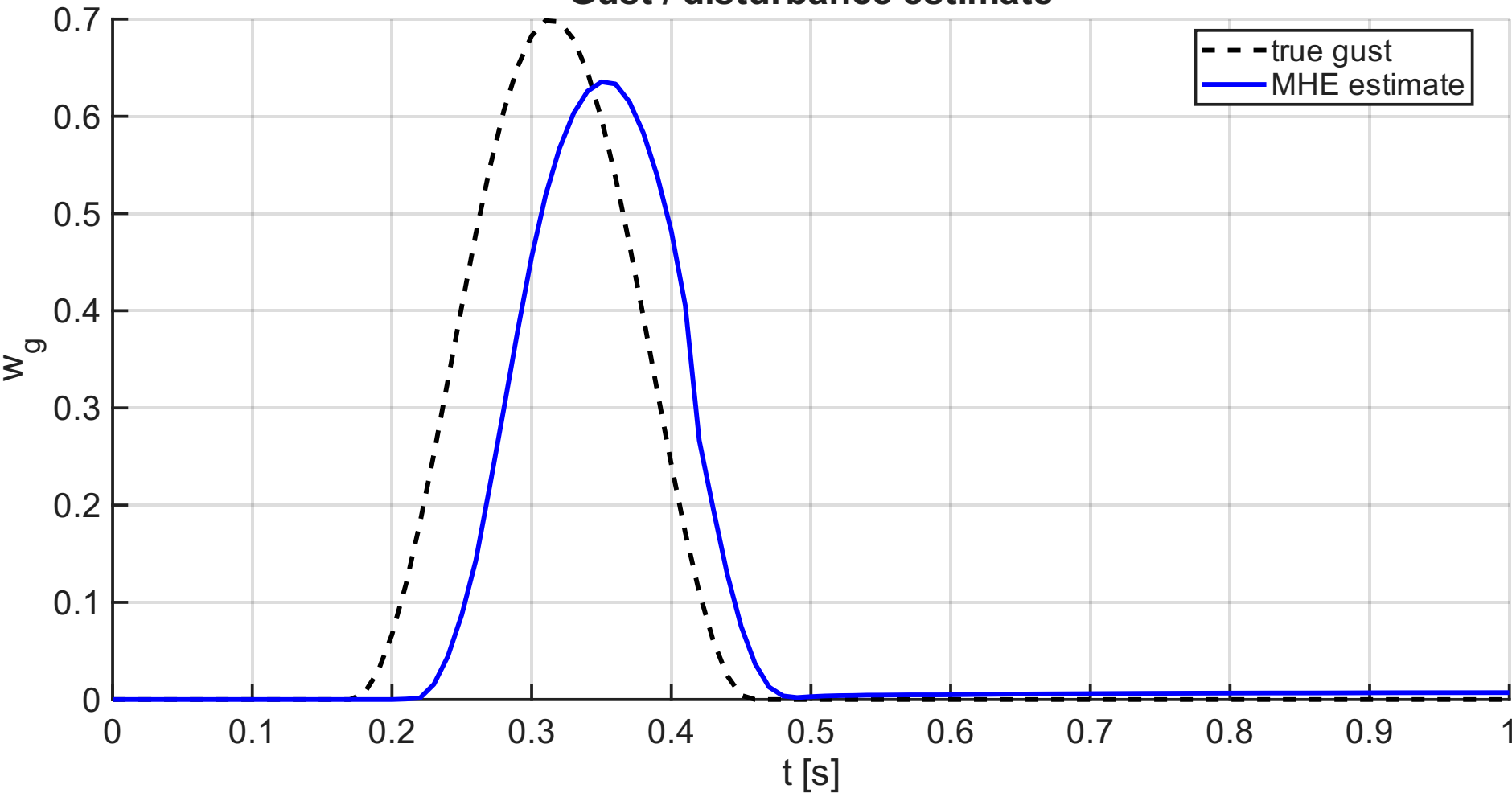
Gust / disturbance estimate
