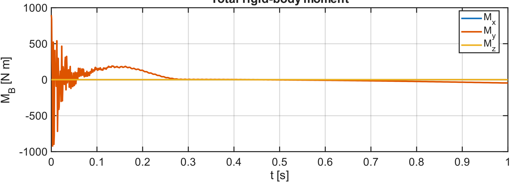
Total rigid-body moment
