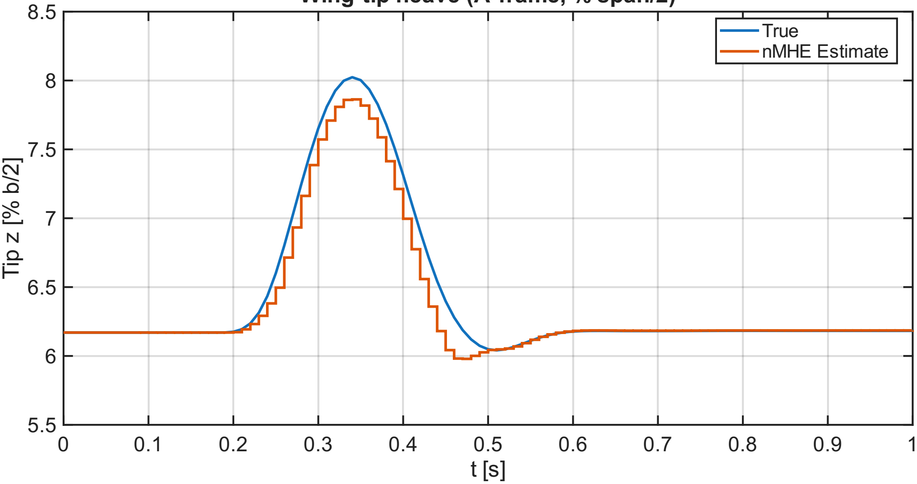
Wing-tip heave (A-frame, % span/2)
